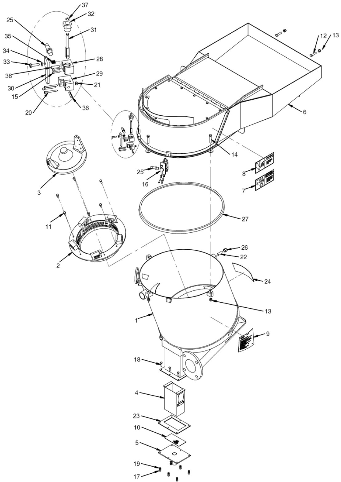
FIGURE 2 - UPPER ASSEMBLY
