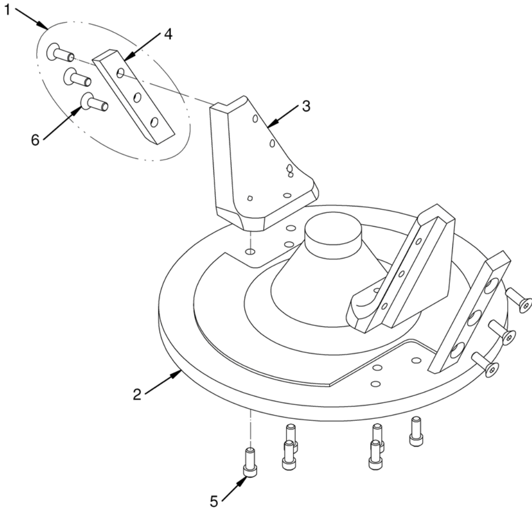
FIGURE 10 –IMPELLER ASSEMBLY
